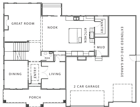
MAIN FLOOR
