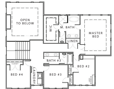
UPPER FLOOR
