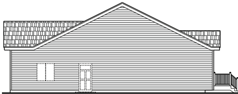
LEFT ELEVATION
