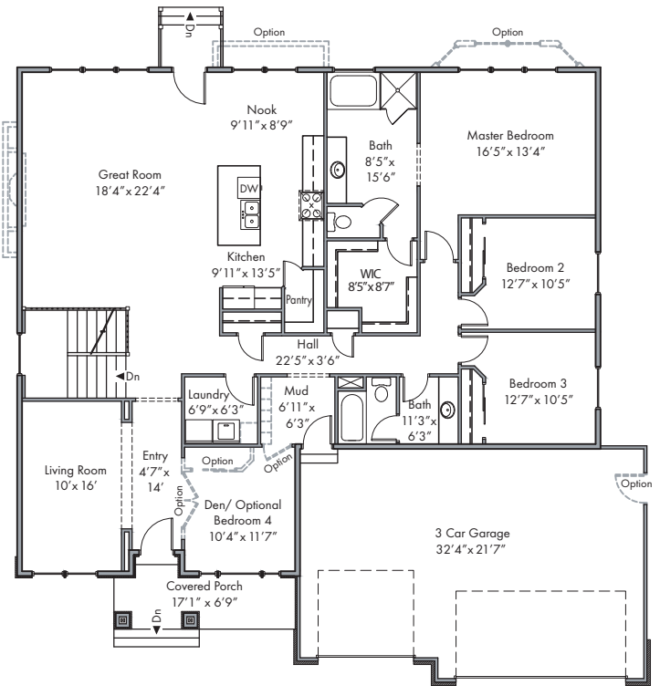
MAIN FLOOR
