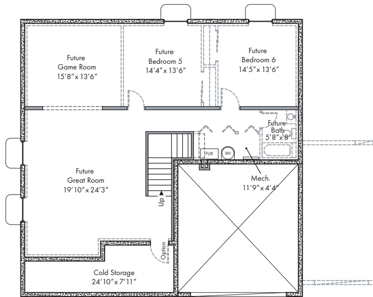
BASEMENT
