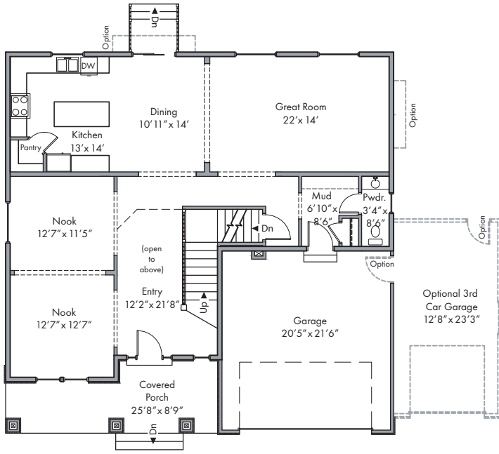
MAIN FLOOR
