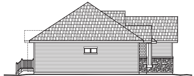
LEFT ELEVATION
