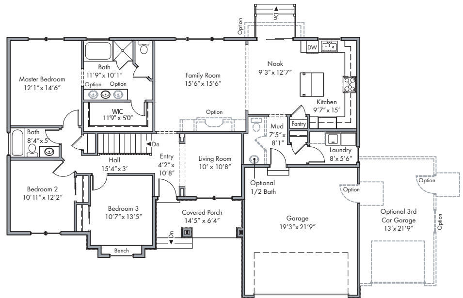
MAIN FLOOR
