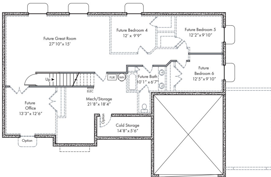
BASEMENT
