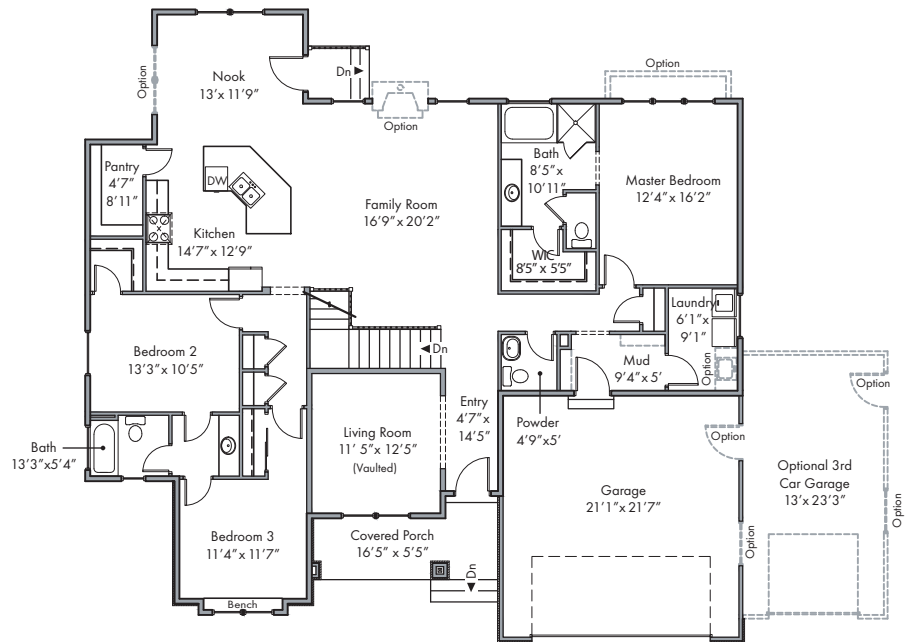
MAIN FLOOR
