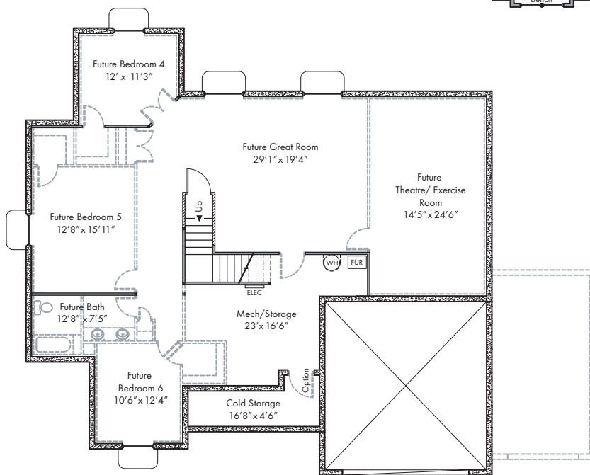
BASEMENT
